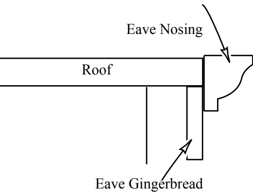
Cross section of Eave Gingerbread and Nosing
